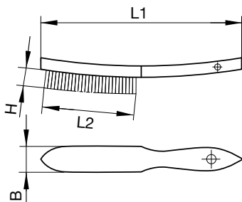
Dimensions brosses manuelles
